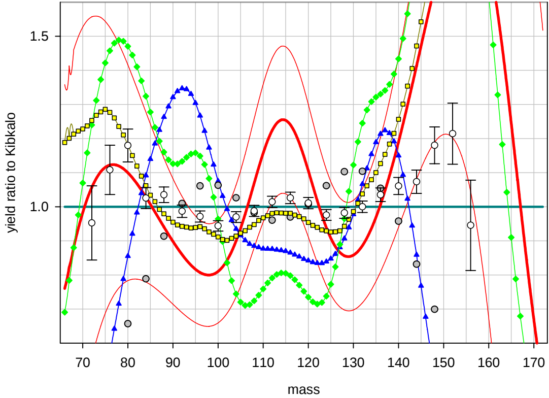
Benchmark A: ^{238}\text{U} at 100 MeV, post neutron emission yield ratio to Kibkalo Lower graph: partial plot (very high and low values omitted); for legend see upper graph.
